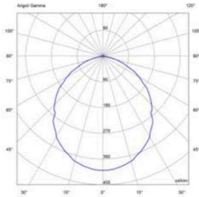
MFN-25-CLN-NW-xx-01-xx 01 (120°) NW 2900lm 80%
