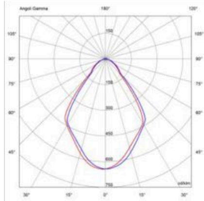
LF-010-MRCS-NW-WHT NW 1270lm WHT (79°) 87%
