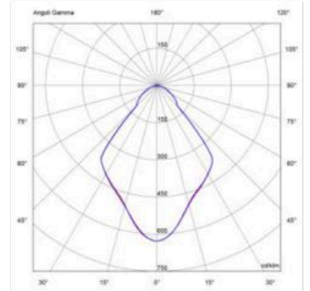
LF-006-MRCS-NW-GLD NW 550lm GLD (80°) 63%
