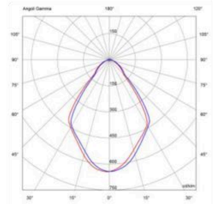
LF-010-MRCS-NW-GLD NW 1270lm GLD (80°) 60%
