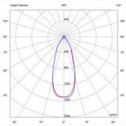
LF-010-MRCS-NW-MFL NW 1270lm MFL (40°) 85%
