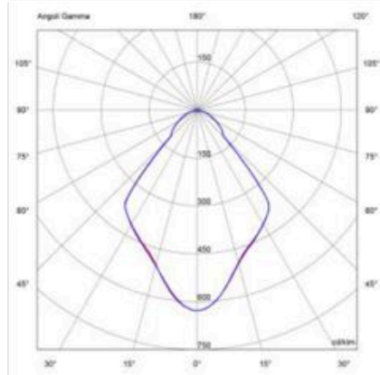
LF-006-MRCS-NW-WHT NW 550lm WHT (79°) 91%
