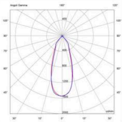
LF-006-MRCS-NW-MFL NW 550lm MFL (40°) 87%
